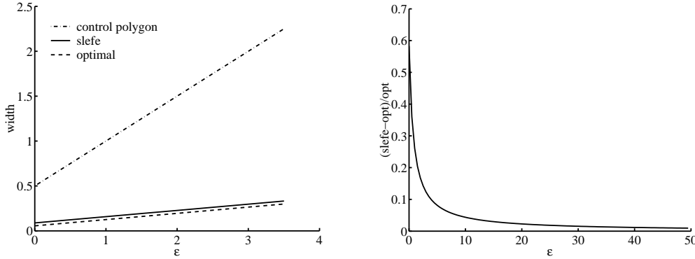
Fig. 7. Cubic f with inflection: ( left ) Value of w_{\text{slefe}}(f; U) , w_{\text{opt}}^{\sim}(f; U) and the width based on the convex hull of the control polygon. ( right ) The ratio \frac{w_{\text{slefe}} - w_{\text{opt}}^{\sim}}{w_{\text{opt}}^{\sim}}(f; U) .
