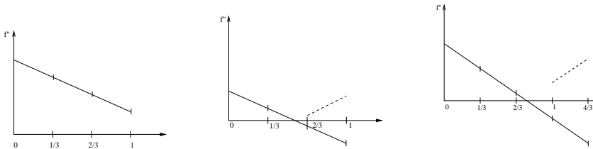
Fig. 5. (left) Linear f'' > 0 , (middle) inflection in the middle segment, (right) inflection in the right segment (middle segment with respect to U' := [1/3..4/3] ) .
