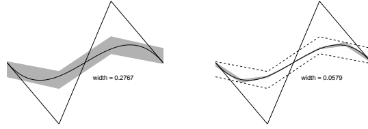
Fig. 2. (left) A cubic Bézier segment with coefficients 0, -1, 1, 0 . The control polygon exaggerates the curve far more than the grey 3-piece slefe. (right) After one subdivision at the midpoint, the width of the slefe ( grey ) is roughly 1/4th of the width of the unsubdivided slefe ( dashed ).
