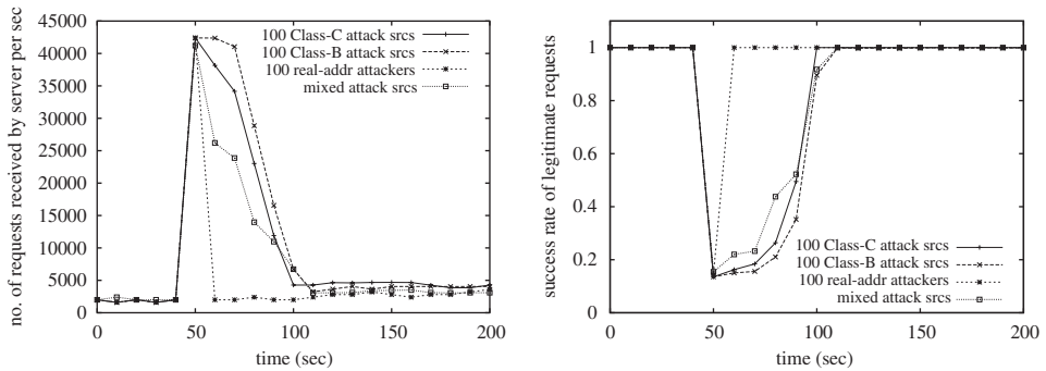
Fig. 3. Defend against DDoS by targeted filtering.
