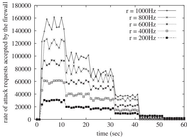
Fig. 9. Experiments with varied attack rates ( r ).
