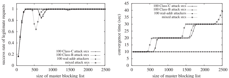
Fig. 5. Impact of different sizes of master blocking list.
