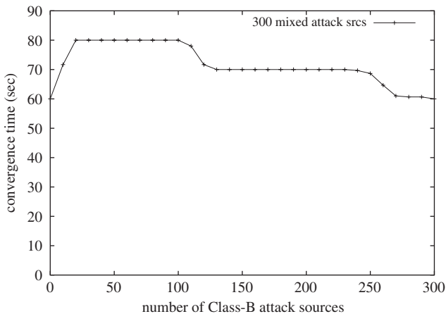
Fig. 7. Mixed attack sources.
