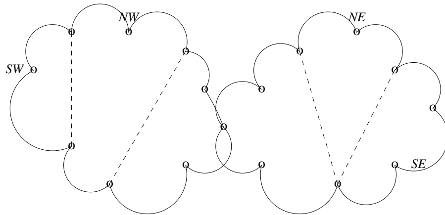
(c) 2 critical corner implying paths
