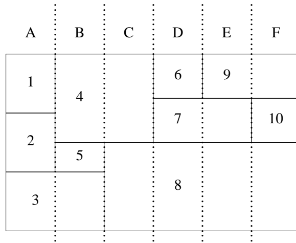
(a) Rectangular dual
