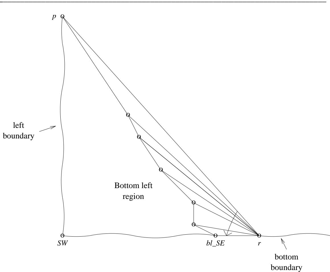
Figure 4.7: Bottom left corner.
