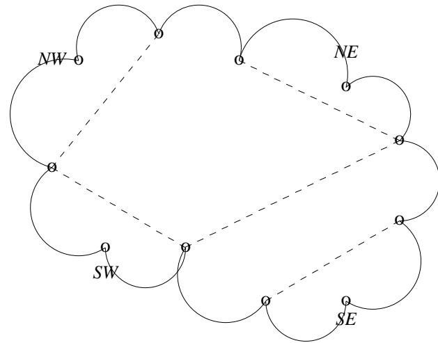
(b) 4 corner implying paths
