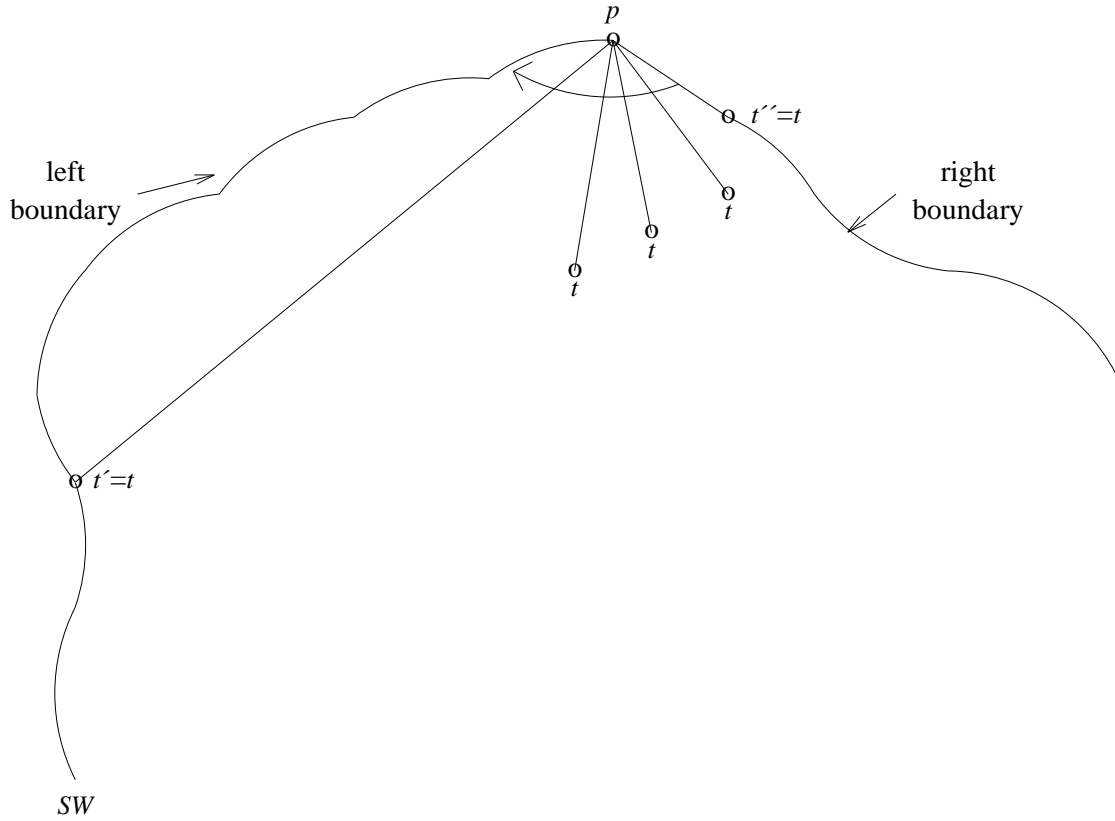
Figure 4.9: Region below p .
