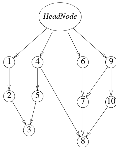
(b) Path digraph
