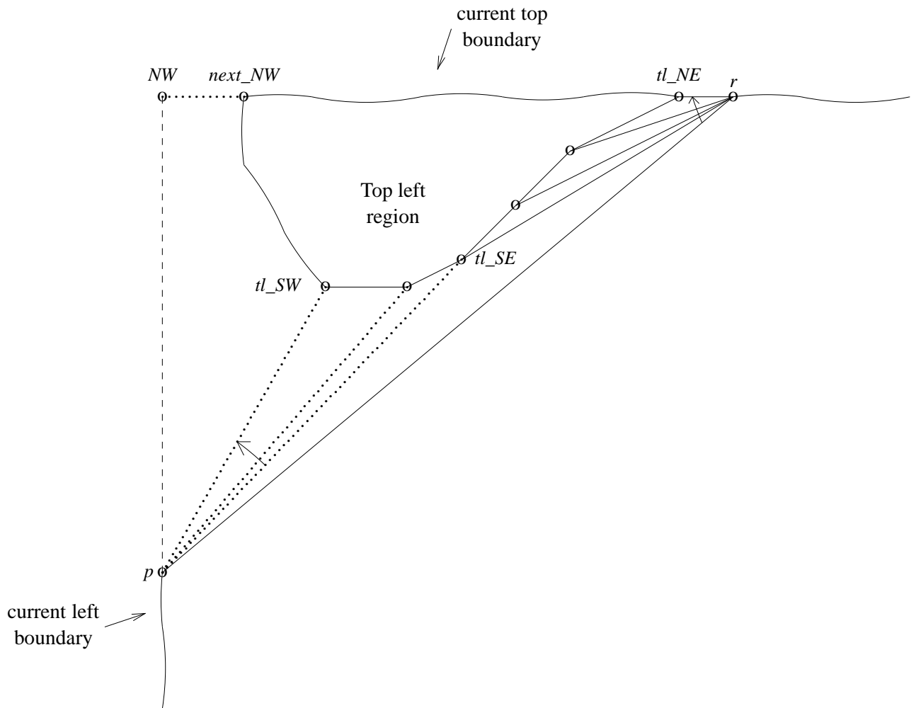
Figure 4.12: Top left region.
