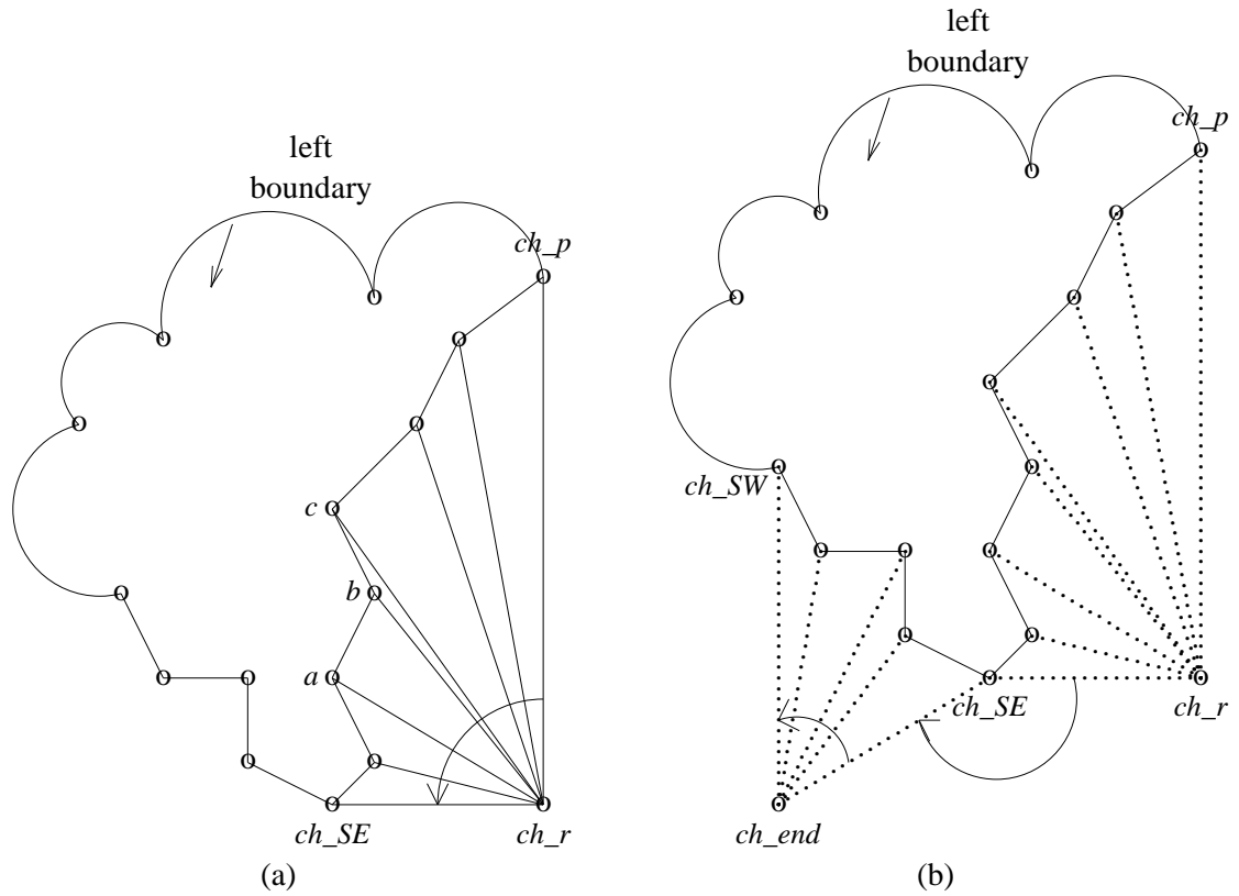
Figure 4.5: Chord (ch_p, ch_r) .
