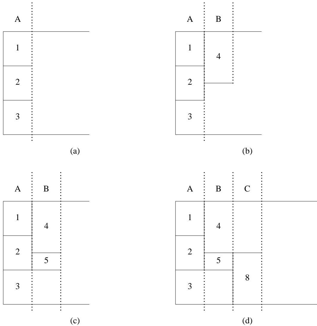
Figure 2.4: Rectangular dual construction. (Continued on next page)
