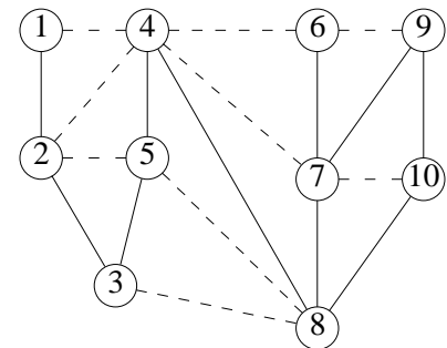
(c) Planar triangulated graph
