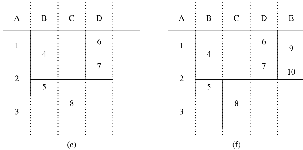
Figure 2.4: Rectangular dual construction. (Contd.)
