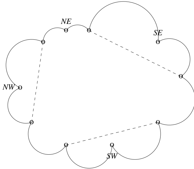
(a) 3 corner implying paths
