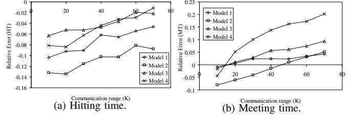
Fig. 6. Relative error between theory and simulation values.
