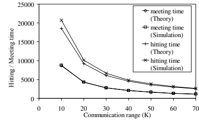
Fig. 5. Comparing the simulation results and theoretical values for the hitting and the meeting times (model 1).
