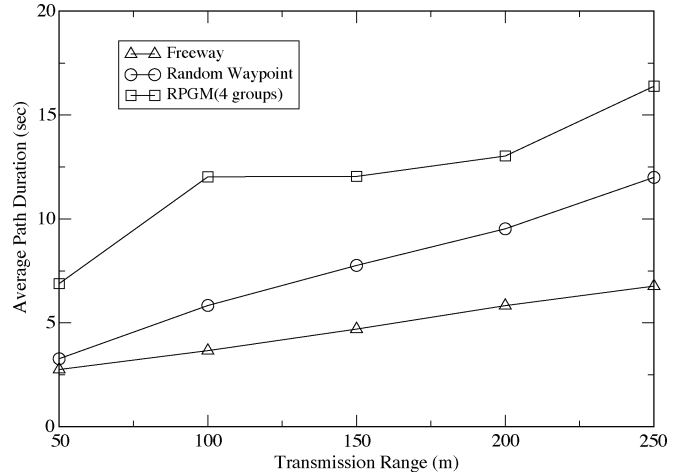
Fig. 20. Effect of R on the average path duration for h = 2 and V_{\max} = 30 m/s (linear relationship).
