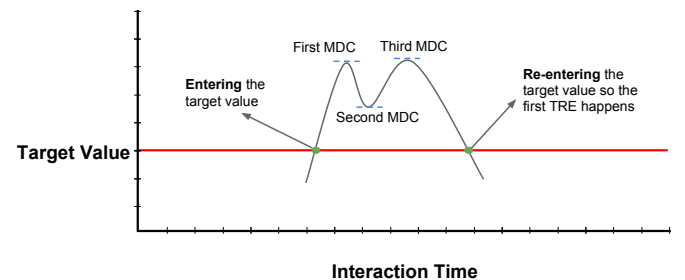
Fig. 7. This indicates part of a line chart used to visualize the interaction log for a particular user. This part of the interaction log enters the target value, leaves, and re-enters once. In this case, there is one target re-entry (TRE), and three movement direction changes (MDC).
