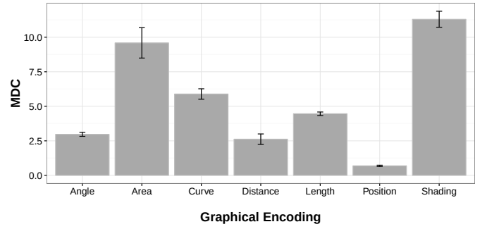
Fig. 8. Means and standard deviations of TRE and MDC for each interactive graphical encoding . The units in this table are “mean count per participant” for TRE and MDC. Error bars represent standard error.
