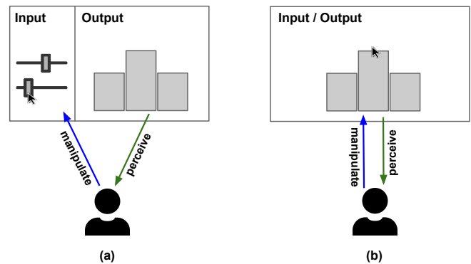
Fig. 1. Two different forms of interaction in many visualization systems. In order to interact with the visualization, users are required to either manipulate the external components in a separate panel (a) or directly manipulate the visual elements (b).
