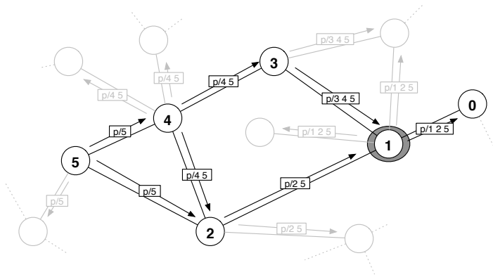
Figure 1: BGP Path discovery - AS5 originates the prefix p by announcing it to its neighbors (e.g., AS4). AS4 further propagates the prefix to its neighbors AS2 and AS3 after prepending its AS number to the prefix. AS1 (highlighted) receives routes from AS2 and AS3, and selects the best route (arbitrarily \{2\ 4\ 5\} ), which is then propagated further (to AS0 and others).
