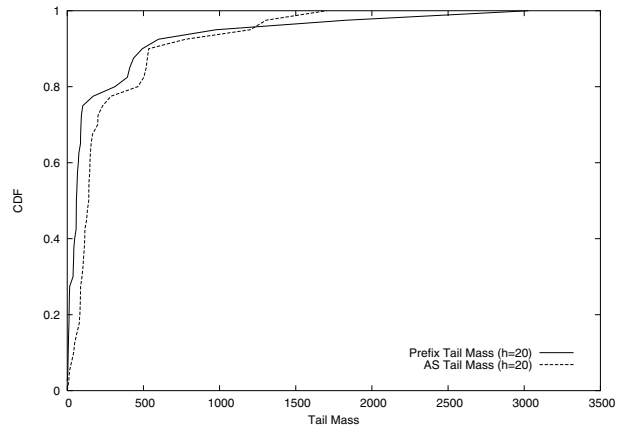
Figure 3: Tail mass - CDF of tail mass for 40 Route Views listening points during February 2004.
