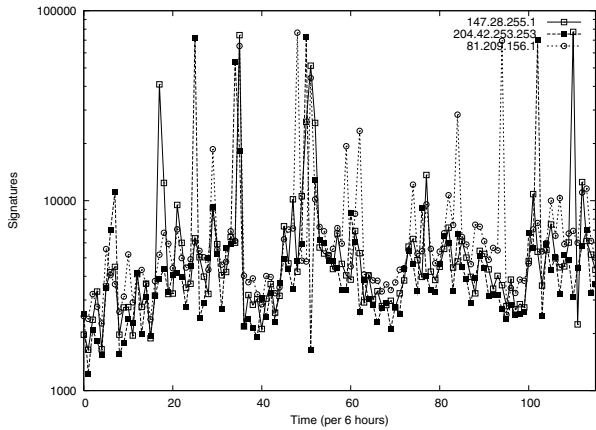
Figure 9: Signature validations by listening point - validations for the origin paths scheme per 6 hour period.
