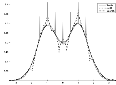
(h) The fixed BW KDE has a lower ISE than the KDE on this double claw density but it misses all the sharp peaks.
