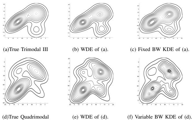
Figure 5. 2D Density estimation comparison: WDE versus KDE contours. See Table II for WDE estimation parameters.
