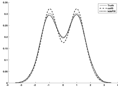
(a) Fixed BW KDE performs slightly better than our WDE on this bimodal density.
