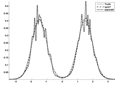
(d) Variable BW KDE has lower ISE than fixed BW KDE in (c) but incorrectly gives several peaks.
