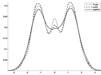
(b) The WDE captures the middle peak of this tridmodal density. The fixed BW KDE misses it.
