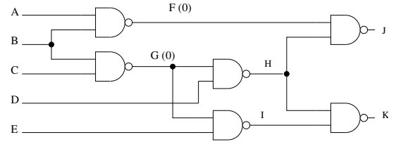
(a) The netlist of c17.
