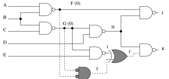
(b) The netlist of c17 with Trojan inserted.
