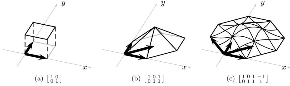
Figure 4. Construction of the ZP-element via directional convolutions.
