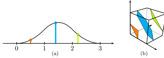
Figure 3. Geometric definition of the box-spline with the direction matrix \Xi := [1 \ 1 \ 1] ; area of intersection of a cube with \Xi^{-1}\{x\} = [1 \ 1 \ 1]^t / 3\{x\} + H_j^2 , the translates of the hyperplanes orthogonal to \mathbf{j}_3 := [1 \ 1 \ 1]^t .
