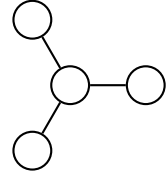
Figure 7. Coxeter diagram of the root system \mathcal{D}_4 .
