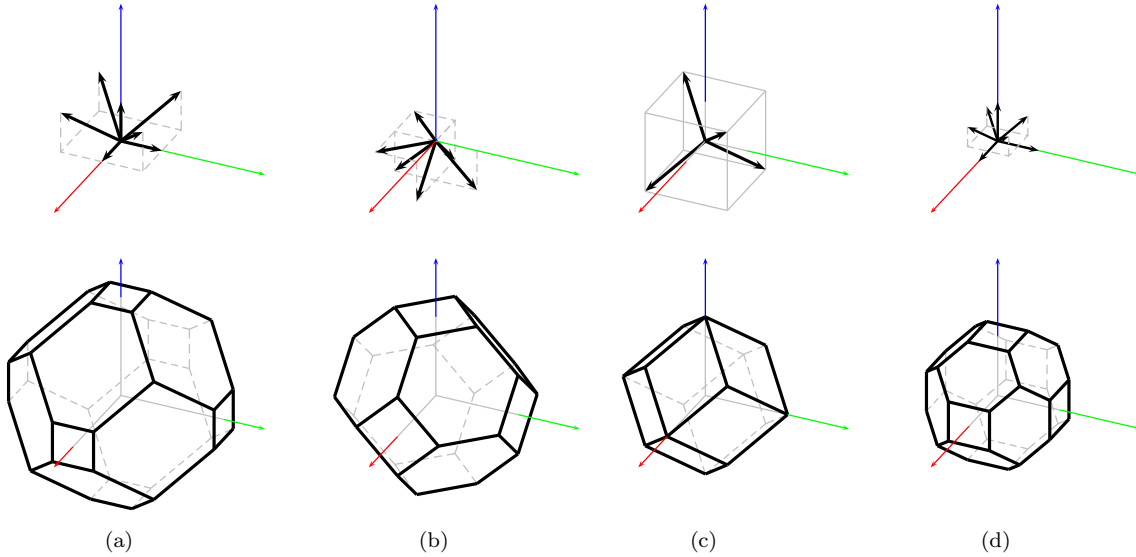
Figure 8. Trivariate symmetric box-splines (top) directions (bottom) supports. (a) 7-direction box-spline on \mathbb{Z}^3 (Section 3.2) (b) 6-direction box-spline on the FCC lattice (Section 5.2 and Section 7.2), (c) 4-direction box-spline on the BCC lattice (Section 6) and (d) 7-direction box-spline on the BCC lattice (Section 8.2).
