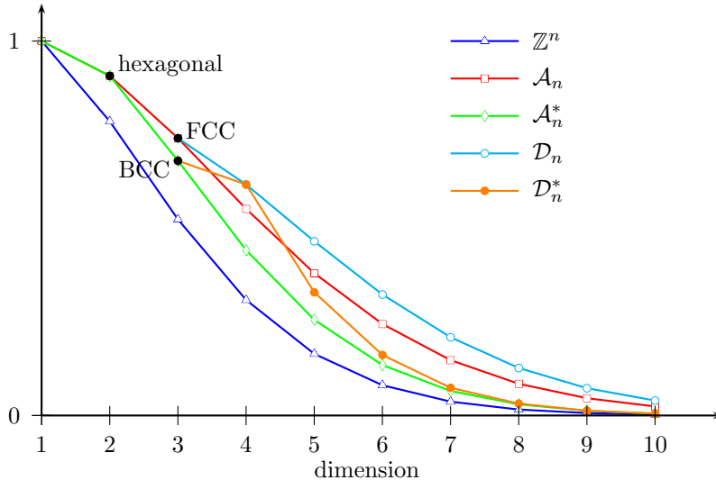
Figure 1. Density of root lattices up to dimension 10. The relative density of \mathbb{Z}^n compared to \mathcal{D}_n for n = 3, 4, 5, 6 decreases as 71%, 50%, 35%, 25%, respectively.
