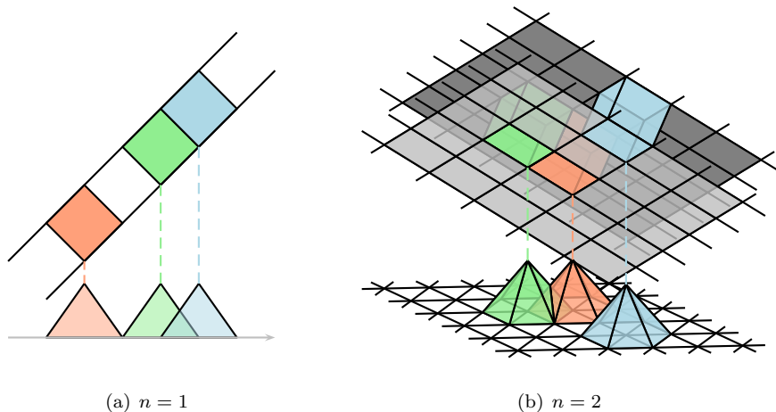
Figure 6. Orthogonal projection of unit cubes along the diagonal direction for (a) n = 1 and (b) n = 2 . [23]
