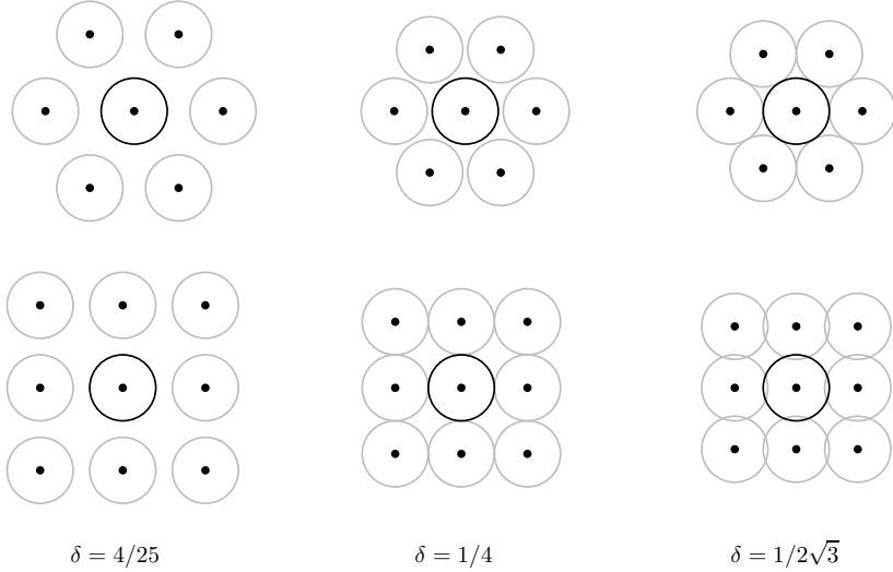
Figure 2. Unit ‘ball’ (primary spectrum and its replicas) packing with respect to the density \delta for (top) the hexagonal lattice and (bottom) the Cartesian lattice. (left) Sampling density is high enough so that no pair of spectra overlap; (bottom center) the primary spectrum and its replicas touch on the Cartesian lattice but (top center) are separated on the hexagonal lattice; (top right) the balls only touch on the hexagonal lattice, and hence the original signal still can be reconstructed without aliasing. (bottom right) On the Cartesian lattice the spectra overlap, causing aliasing.
