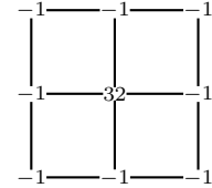
Figure 5. Quasi-interpolation stencil of M_{\mathbb{Z}^2} (scaled by 24).
