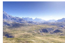
Fractals
