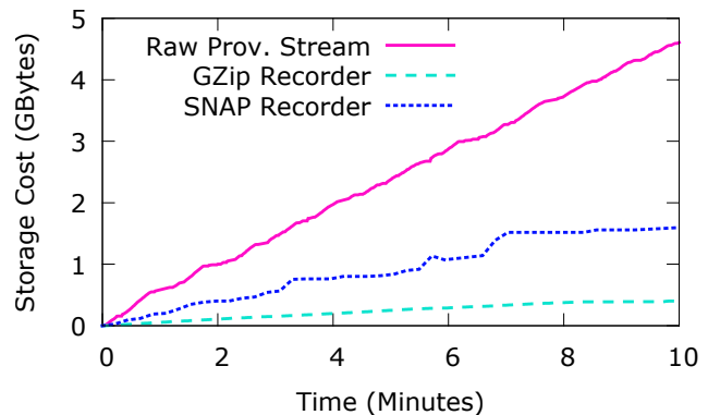
Figure 1: Growth of Hi-Fi’s provenance log during kernel compilation using different LPM storage backends. Log growth is only manageable when compressed with gzip , but in this form it cannot be efficiently queried.
