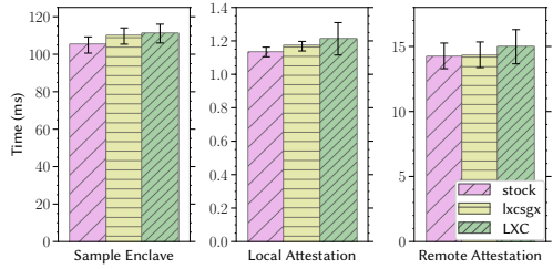
(a) Timing in ms of three simple SGX applications provided in the Intel SGX SDK in three settings (1) stock kernel, (2) lxcsgx kernel, and (3) LXC.
