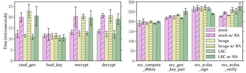
(b) Timing in \mu s of 8 TPM commands provided by tpmsgx . Commands were run, both with and without remote attestation (RA) enabled, in three settings: (1) stock kernel, (2) lxcsgx kernel, and (3) LXC.
