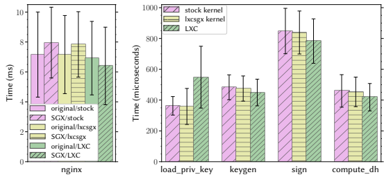
(c) Timing in ms of original Nginx and SGX version with sgxengine communicating with tpmsgx (left); timing in \mu s for 4 operations in Nginx, each run in three settings (right).
