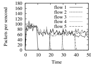
Fig. 12: AdjConWin
