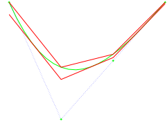
Fig. 3. a := \mathbf{a}_1^3 := -(2\mathbf{b}_1^3 + \mathbf{b}_2^3)/3 with control polygon and slefe.
