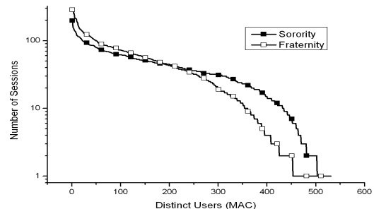
Figure 1: Session count for Sorority and Fraternity users
