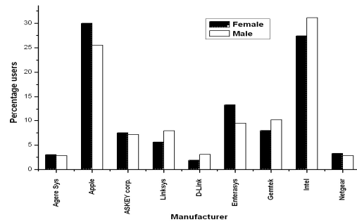
Figure 4: Device distribution by manufacturer
