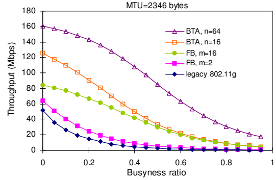
Figure 7. Theoretical throughput of Frame-bursting and Block ACK schemes with different burst sizes
