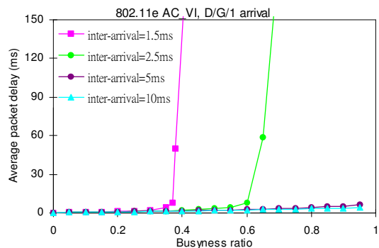
Figure 6. Theoretical delay limit of 802.11e AC_VI with different arrival process
