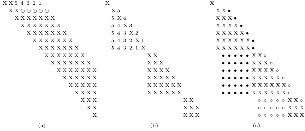
Fig. 8. Update of U . (a) Upper triangular part of symmetric matrix A (b) U after reducing entries 1 \dots 5 (c) U after reducing \oplus entries.
