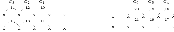
Fig. 4. Applying column rotations to C-block.
