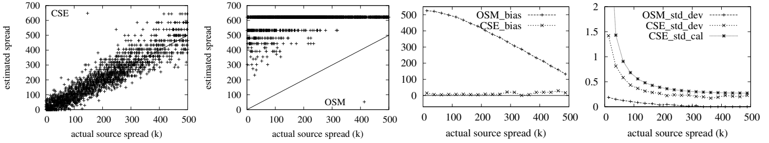
Fig. 3. m = 0.5\text{MB} . Each point in the first plot (CSE) or the second plot (OSM) represents a source, whose x coordinate is the true spread k and y coordinate is the estimated spread \hat{k} . The third plot shows the bias of CSE and OSM, which is the measured E(\hat{k} - k) with respect to k . The fourth plot shows the standard deviation, which is the measured \sqrt{\text{Var}(\hat{k})} for CSE and OSM, together with the numerically-calculated standard deviation for CSE based on (26) and (24).
