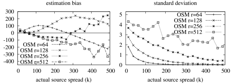
Fig. 8. The left plot shows the bias of OSM, which is the measured E(\hat{k} - k) with respect to k . The right plot shows the standard deviation of OSM, which is the measured \frac{\sqrt{\text{Var}(\hat{k})}}{k} .
