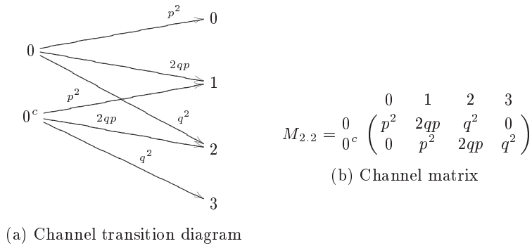
Fig. 6. Channel for Case 2.2.
