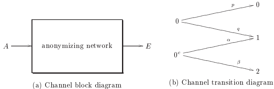
Fig. 4. Channel model for Case 2.1
