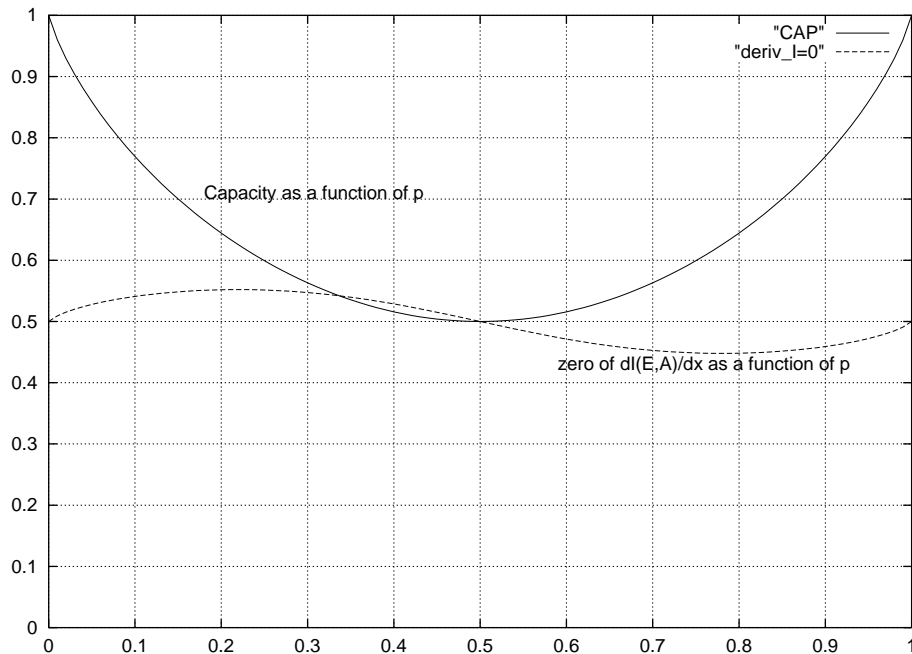
Fig. 5. Plots of covert channel capacity as a function of p , and of the x value that maximizes the mutual information as a function of p .
