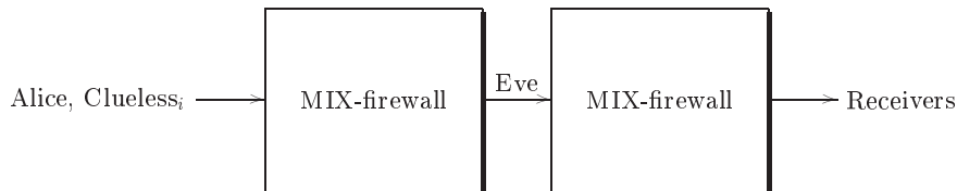
Fig. 3. MIX-firewalls with Restricted Passive Adversary.
