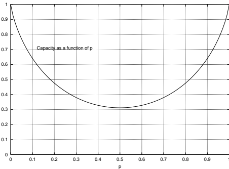
Fig. 7. Capacity as a function of p for Alice with two additional transmitters.
