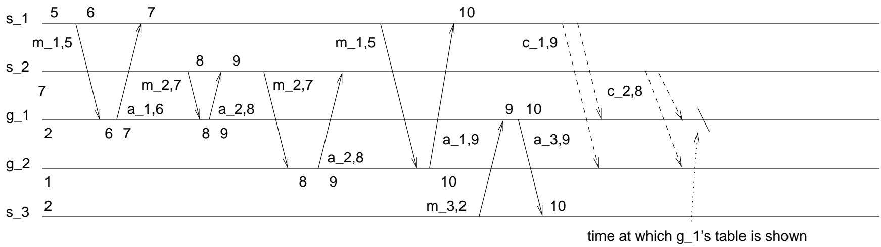
Total Order Multicast Example: Time-Space Diagram
