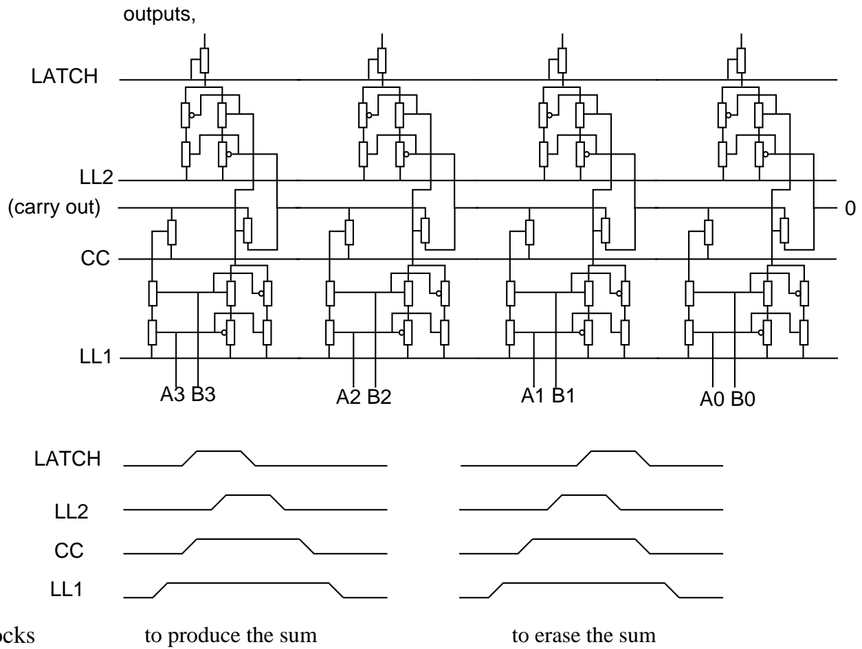
Fig. 9 Retractable cascade adder
