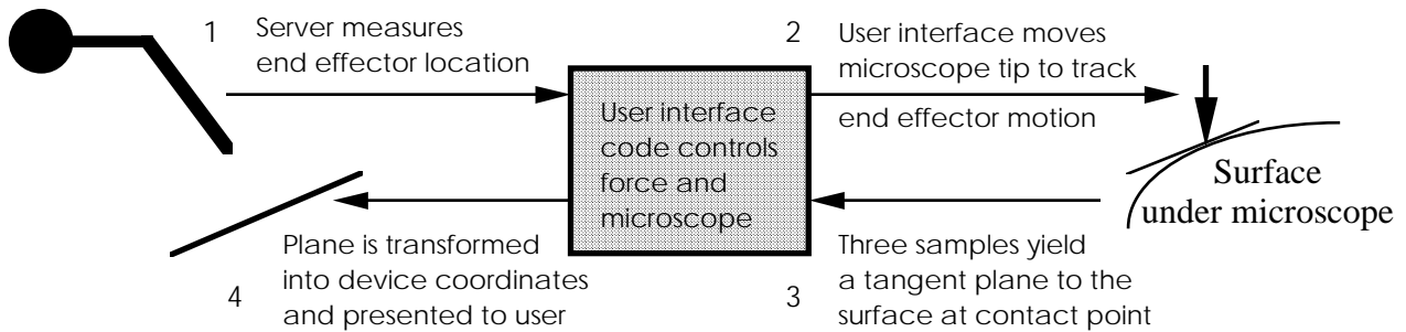
Figure 4: The nanoManipulator application determines a local plane approximation to send to the force server. As the end effector moves, the microscope tip tracks it on the surface and sends a new plane equation describing the local surface.
