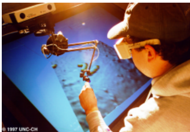
Figure 2: The nanoManipulator application adds a virtual-reality interface to a scanned-probe microscope. Haptic feedback allows the user to feel and modify the microscopic surface.
