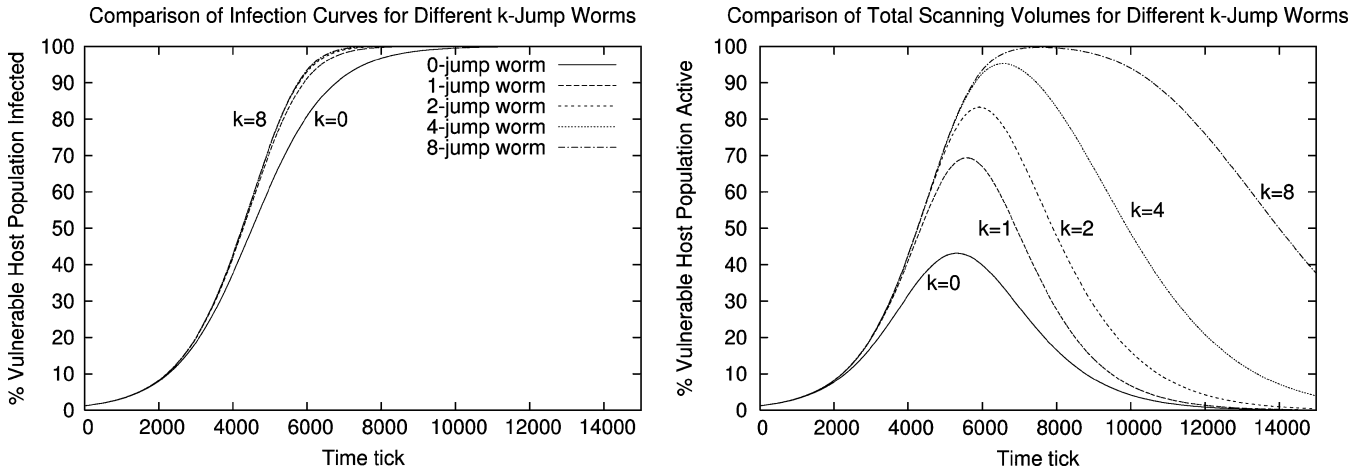
Fig. 7. The left plot shows the infection curves, i(t) , for a k -jump worm under different k values. The right plot shows the active curves, a(t) , for a k -jump worm under different k values. Recall that a(t) is the percentage of vulnerable hosts that are actively scanning at time t . The total amount of scanning traffic, called the scanning volume , is defined as the area under the active curve. From the left plot, we see that the infection speed improves when k increases. However, the rate of improvement diminishes quickly when k is greater than 1. On the other hand, from the right plot, the scanning volume increases significantly when k increases.
