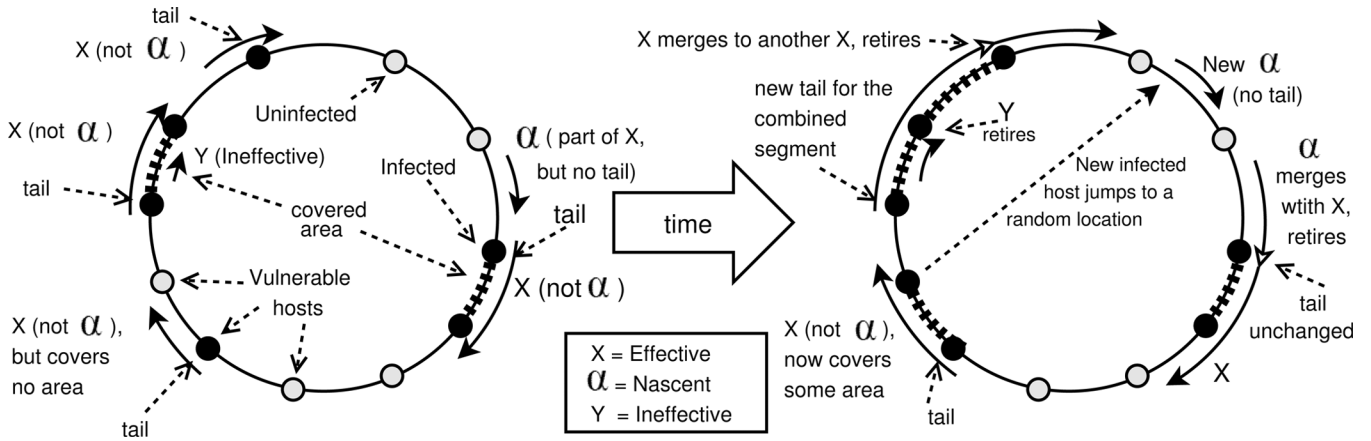
Fig. 1. Depiction of scanzones for a 0-jump worm over time. Scanzones of active hosts are depicted as arcs on the permutation ring. Uninfected and infected vulnerable hosts are depicted as white and dark dots on the permutation ring, respectively.
