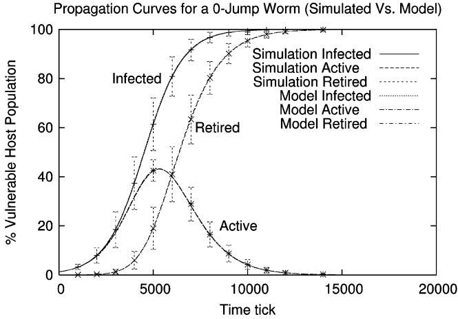
Fig. 4. The “Model” curves show the percentages of vulnerable hosts that are infected , active , and retired over time, respectively. These curves for i(t) , a(t) , and s(t) are numerically computed from the analytical model in (1)–(11). The “Simulation” curves are plotted using the averaged data collected from the simulator; the 99% confidence intervals are also plotted for selected data points. As expected, the curves from the model and the curves from the simulator completely overlap, which verifies the correctness of the model.
