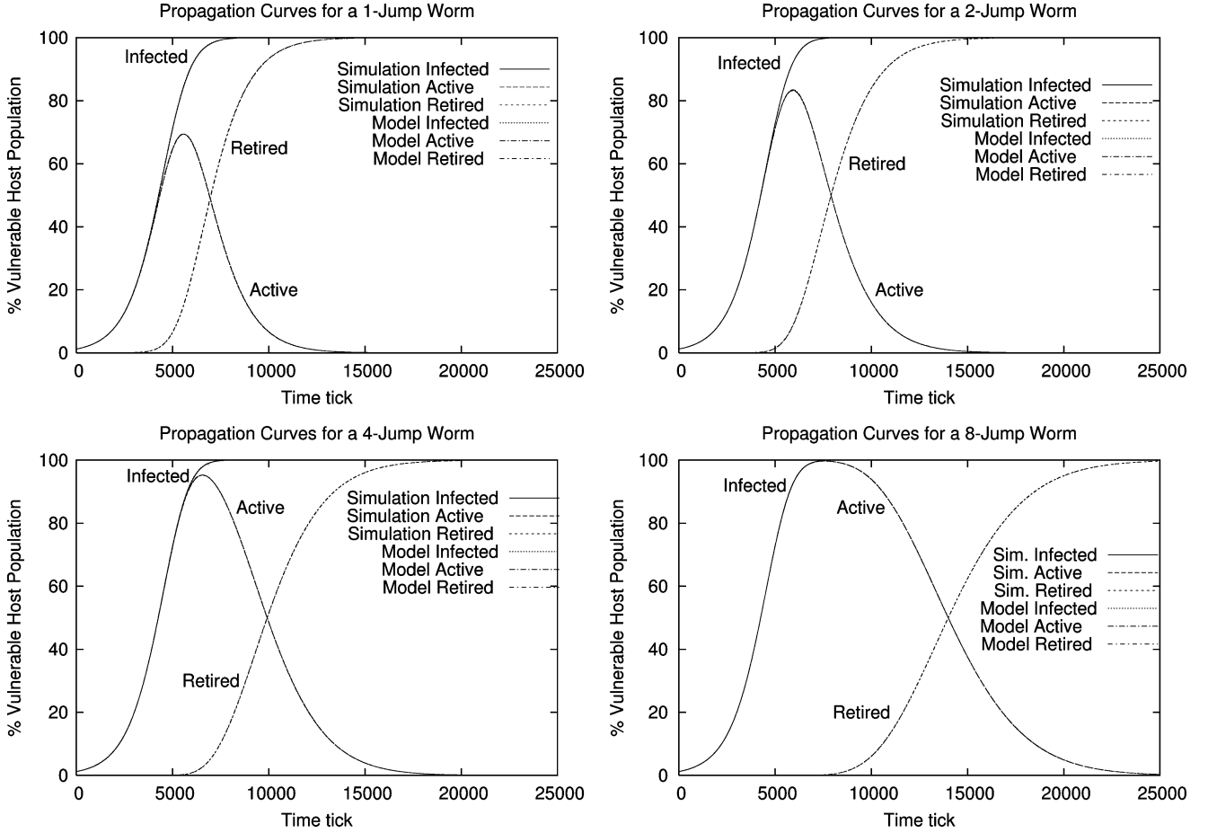
Fig. 6. The “Model” curves show the percentages of vulnerable hosts that are infected, active, and retired over time, respectively. These curves for i(t) , a(t) , and s(t) are numerically computed from the analytical model in (12)–(20). The “Simulation” curves are plotted using the averaged data collected from the simulator. As expected, for k = 1, 2, 4 , and 8 , the curves from the model and the curves from the simulator completely overlap, which verifies the correctness of our model for k -jump worms.
