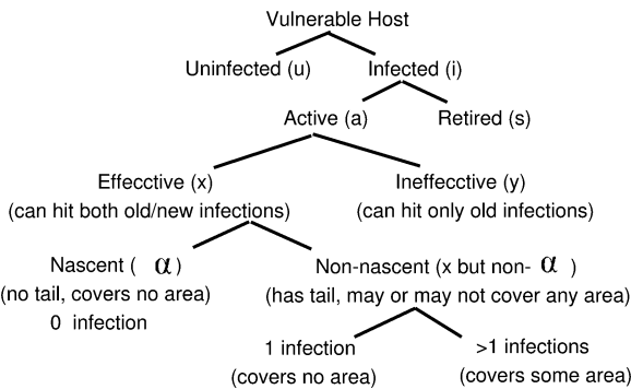
Fig. 2. Classification of vulnerable hosts for a permutation-scanning worm.
