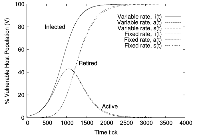
Fig. 8. Comparison of propagation curves for worms with variable- and fixed-rate of scanning. The simulation parameters used are N = 2^{23} , V = 2^{13} , and v = 100 . The value of r is a constant five scans per time tick for the fixed-rate scanning worm, and the other having variable rates with the Gaussian distribution and a mean value of 5 per time tick.
