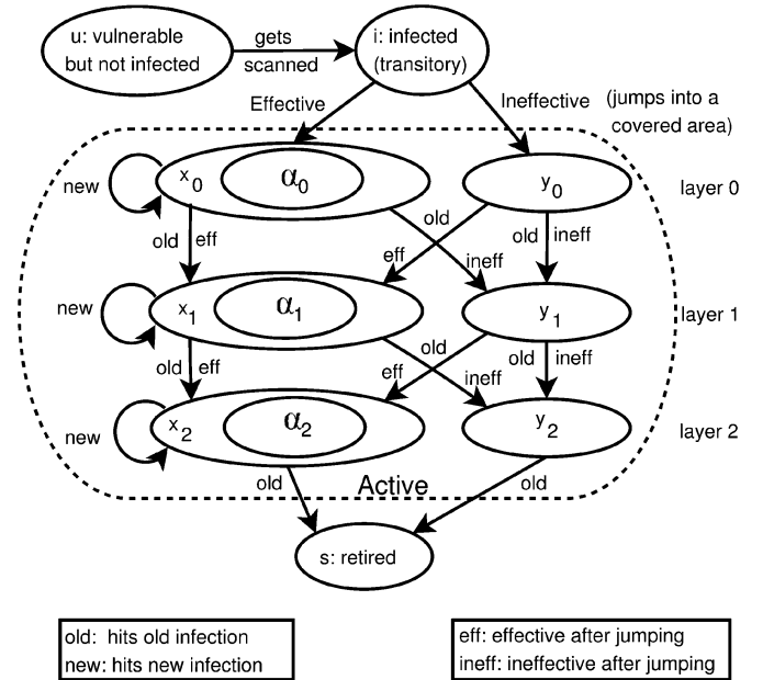
Fig. 5. State diagram of a k -jump worm with k = 2 . In the diagram, we assign each active host a layer number , which indicates the number of old infections hit by the host. Once the host hits its (k + 1) -th old infections, it retires immediately.
