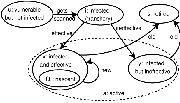
Fig. 3. Class transition diagram of a 0-jump worm. Here, “new” or “old” indicates the event of a new or old infection. Similarly, “ineffective” or “effective” indicates whether the newly infected host, after the random jump, lands in a covered area or not.
