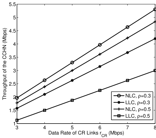
Fig. 5. The throughput performance of the NLC approach and the LLC approach.
