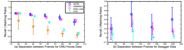
Figure 2. Performance accuracy using the “Recall” measure for non-rigid registration algorithms on the CMU House Sequence (left) and the 3D swagger motion data (right). Legend in (a) is for both sub-figures.
